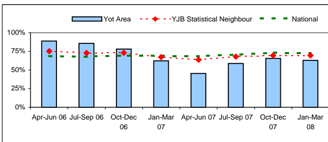
KPI Performance
